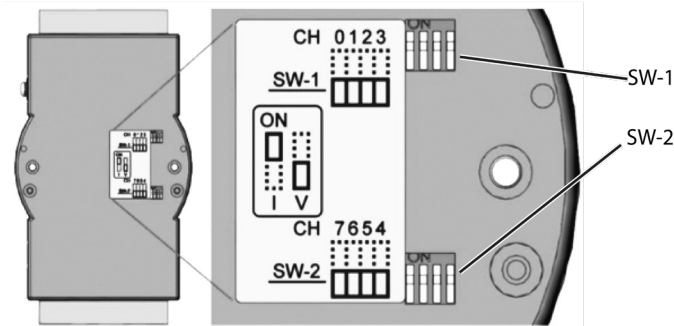
Figure 5: Cut-outs providing access to SW-1 and SW-2 and an illustration map on the back of the Analog Input Expansion Module
