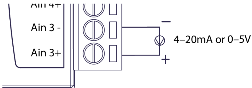
Figure 6: 4–20 mA current loop on Channel 3, where + is the signal from the transducer
