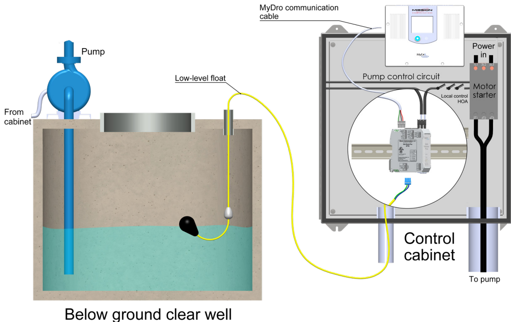
Figure 3: Service pump lock-out application
