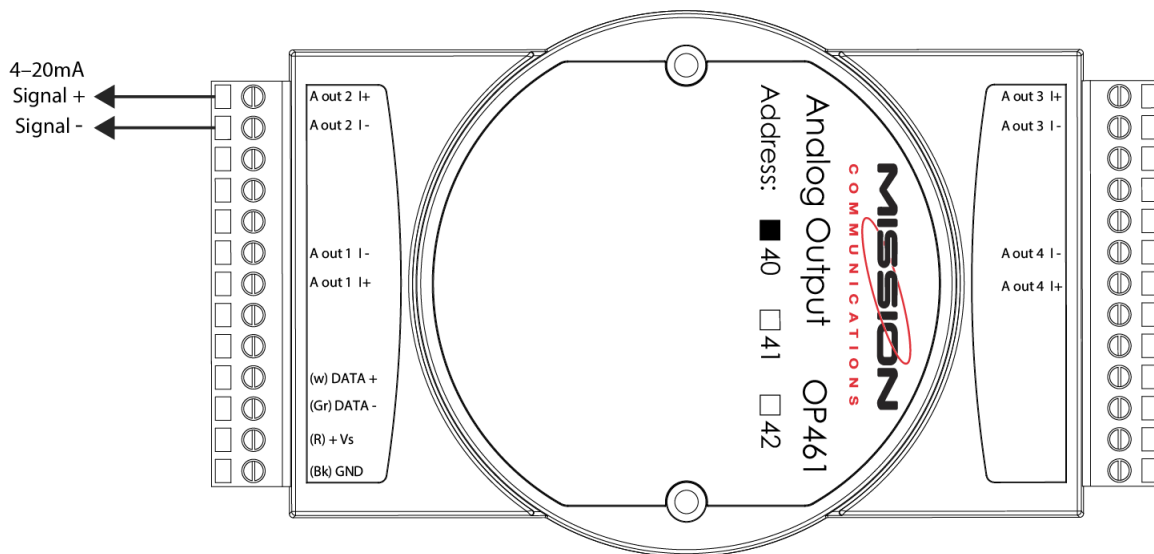
Figure 7: Analog output current loop on output channel 2
