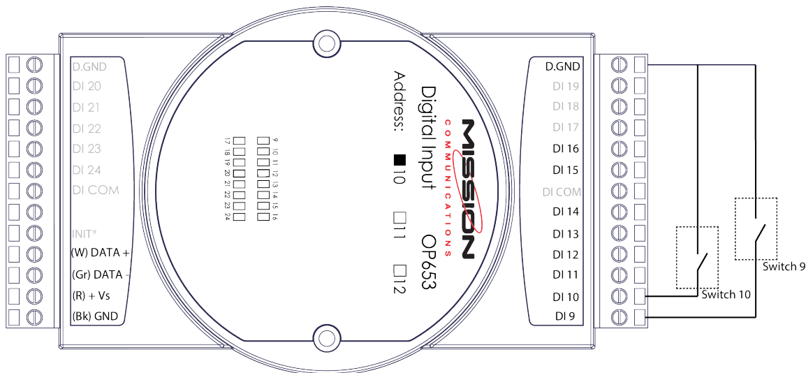
Figure 8: Dry Contact Wiring Diagram Logic level 1: close to GND, Logic level 0: open
